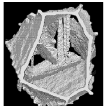
Figure 3: Isosurface.
