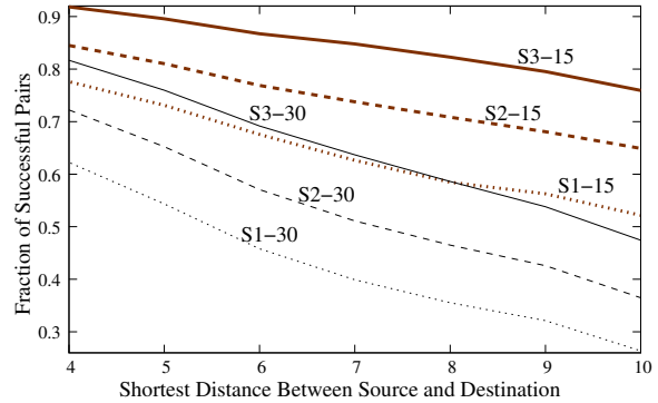
Figure 1. Quantitative measures for the utility of the upstream per-hop hash value.
