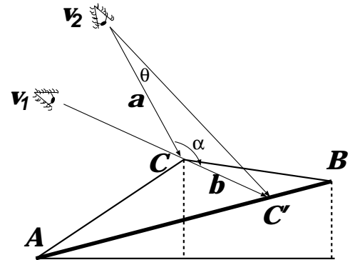
Figure 4: Calculating the error metric.
