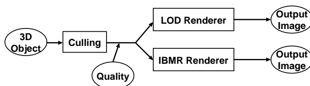
Figure 1: Traditional hybrid LOD and IBMR techniques render each object either as a sprite or at a certain level of detail.
